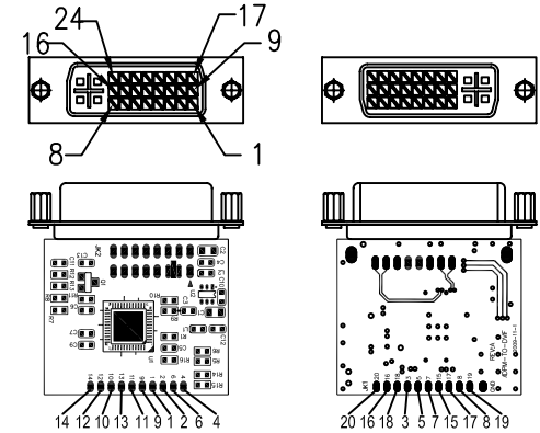
PCB'A DB004-02A
